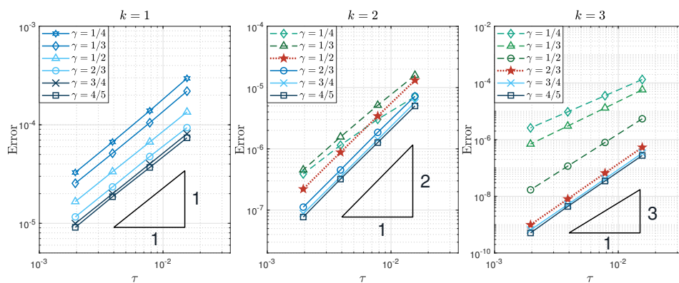
FIG. 4.3. Errors of the numerical solutions at T = 1 for the nonsmooth initial data in (a), with several different parameters \gamma \in (0, 1) .
