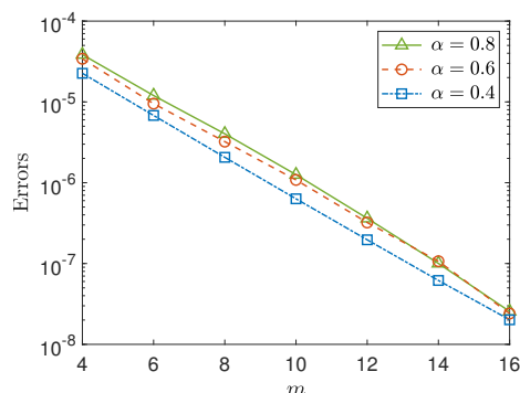
FIG. 5.2. Errors of the numerical solutions for the semilinear subdiffusion equation.
