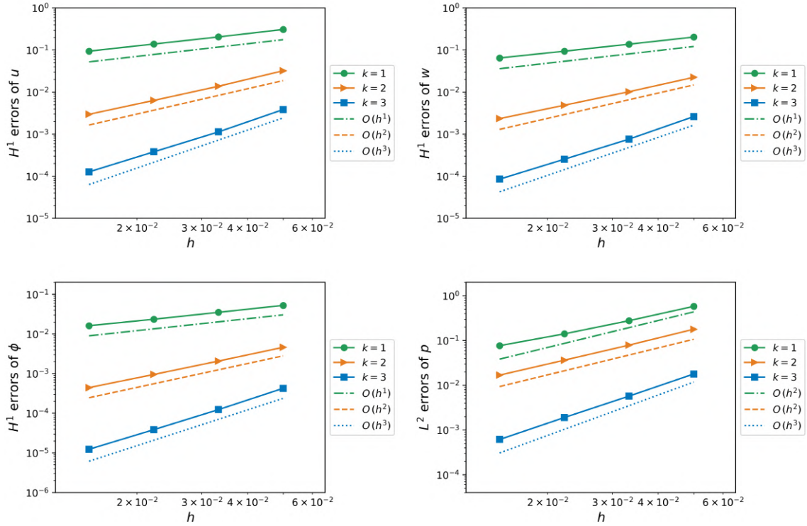
FIG. 3. Spatial discretization errors of the numerical solutions at T = 0.5 .
