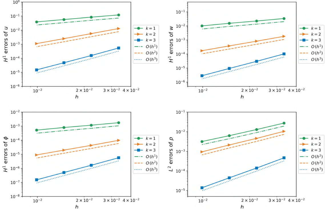
FIG. 2. Spatial discretization errors of the numerical solutions at T = 0.1 .
